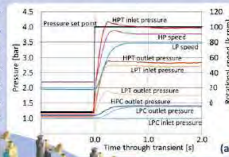
Figure 5. (a) 1-4 bar step response; (b) twin-entry turbine, out-of-phase pulses
