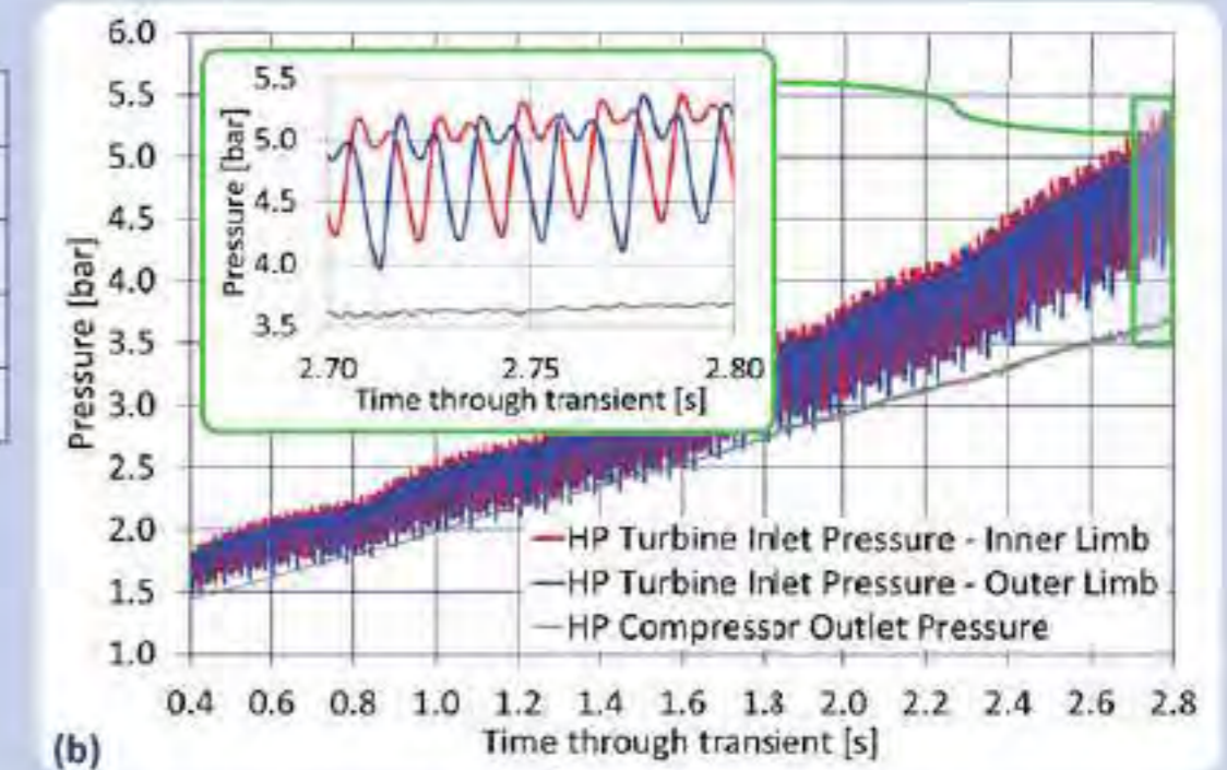
Figure 5. (a) 1-4 bar step response; (b) twin-entry turbine, out-of-phase pulses
